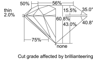
Cut grade affected by brillianteering
